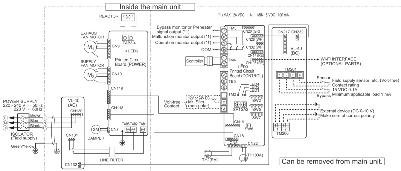
Wiring Diagram
