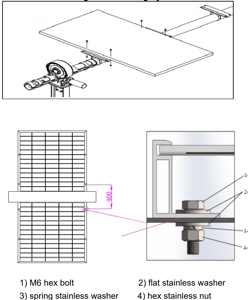
Fig 2. Backsheet-Glass module with Single-axis Tracing System
